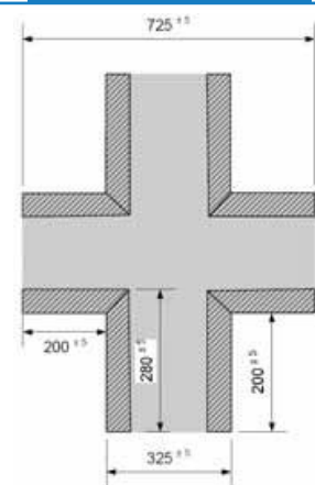
Obr. 9: Mapeband TPE 325 Cross
