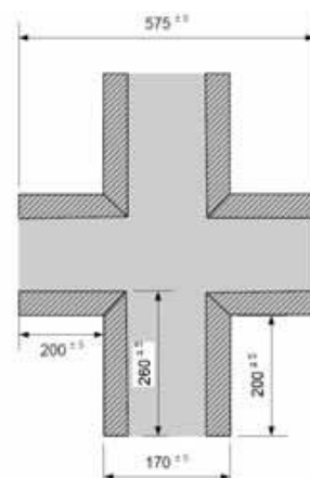
Obr. 7: Mapeband TPE 170 Cross
